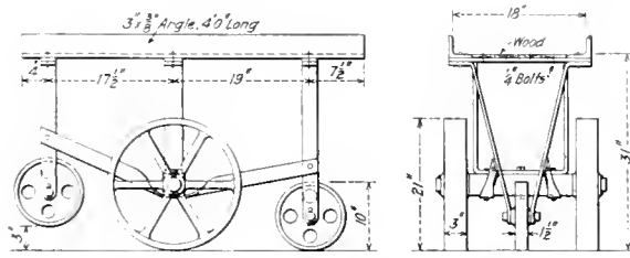
Fig. 3—Wagon for Carrying Locomotive Rods
